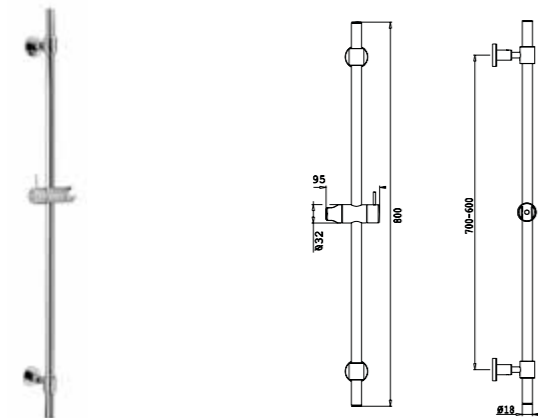
Asta doccia ø 18 mm cursore orientabile L. 800 mm Sliding rail ø 18 mm with adjustable shower holder L. 800 mm
