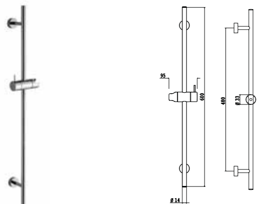
Asta doccia ø 14 mm cursore orientabile L. 600 mm Sliding rail ø 14 mm with adjustable shower holder L. 600 mm
